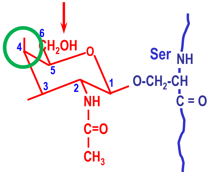
N-acétyl-β-D-galactopyranosamine
