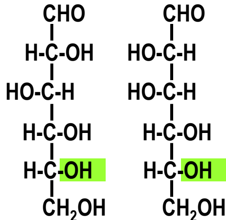
D-glucose
