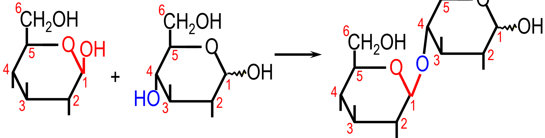
\beta -D-glucopyranose
