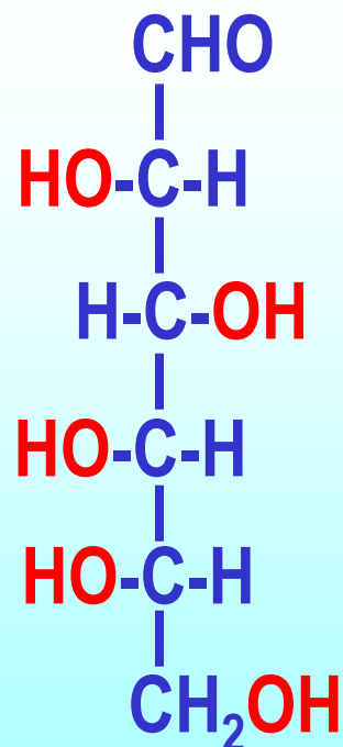
L-glucose
