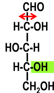
D-xylose
