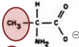
Asparagine (Asn)
